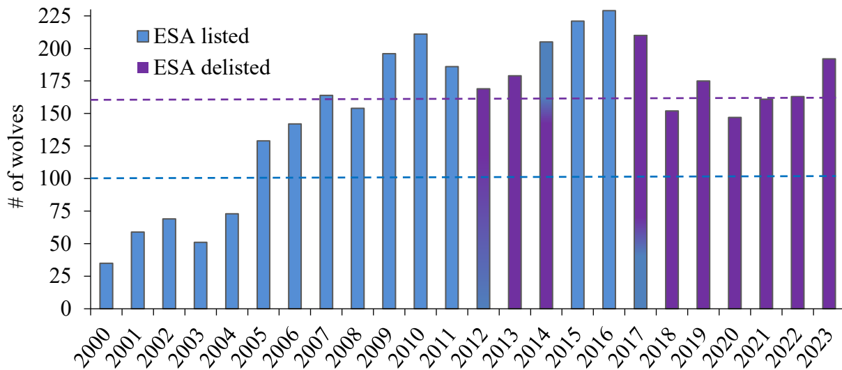
Figure 2. Minimum number of wolves in the WTGMA at the end of the calendar year. (Endangered Species Act status [listed vs. delisted] is included for comparative purposes. The blue dashed line indicates the \geq 100 wolf minimum population commitment; the purple dashed line indicates the 160 wolf population objective for the WTGMA.)
